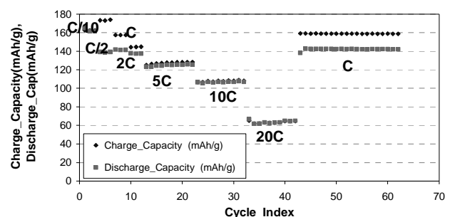
Figure 7: Capacity of CEA Li 4 Ti 5 O 12 vs charge rate
